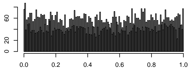
sigma
