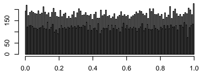
quants_gt
