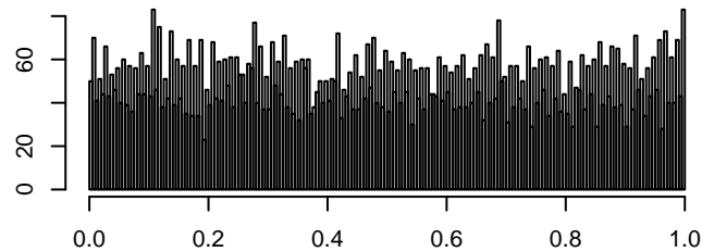
alpha
