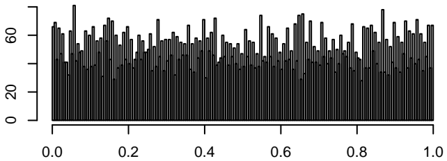
beta
