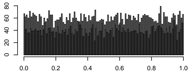
beta
